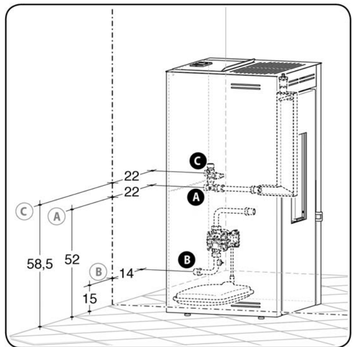
A. Delivery pipe to system (3/4" m) B. Return pipe to system (3/4" m) C. Heat release safety valve (1/2" f - 3 bar)
